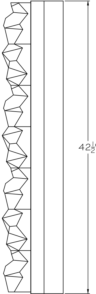
FRONT VIEW
