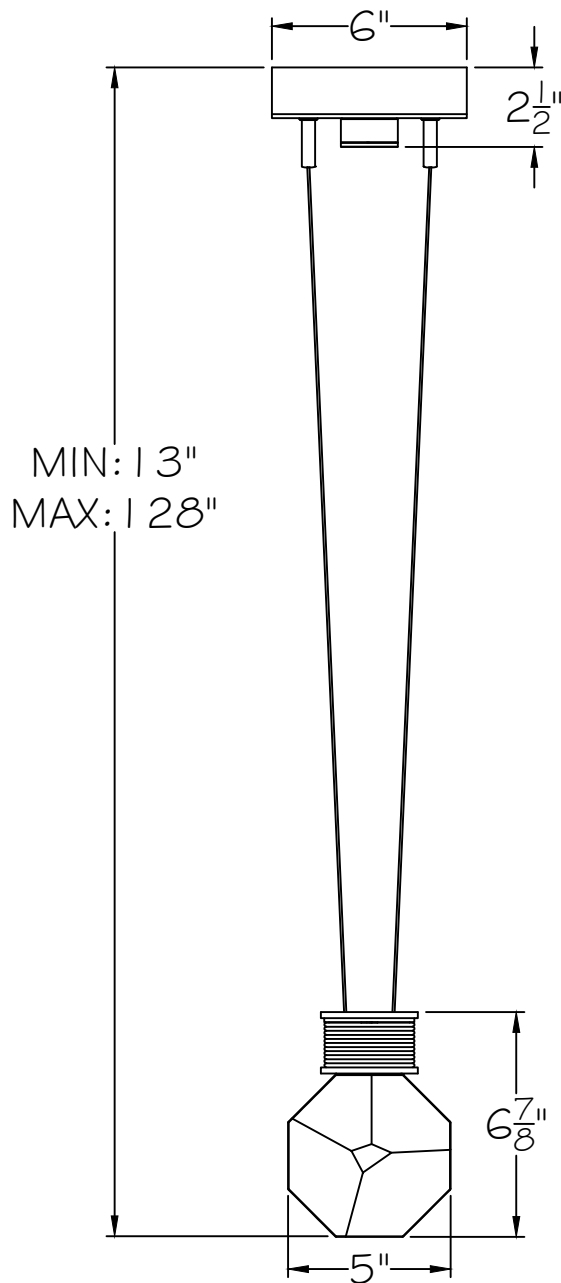
FRONT VIEW
