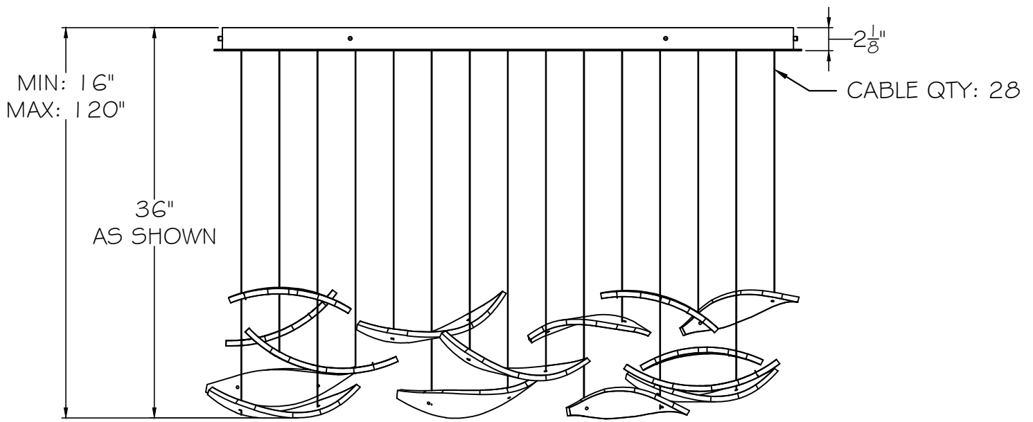
FRONT VIEW
