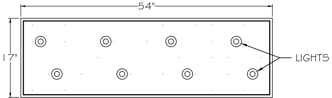
TOP VIEW
