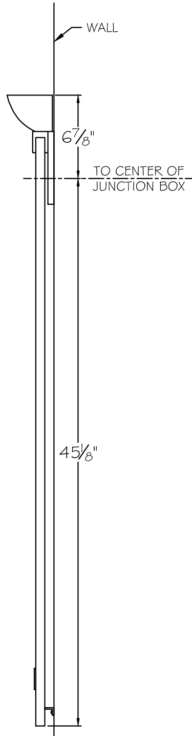
SIDE VIEW
